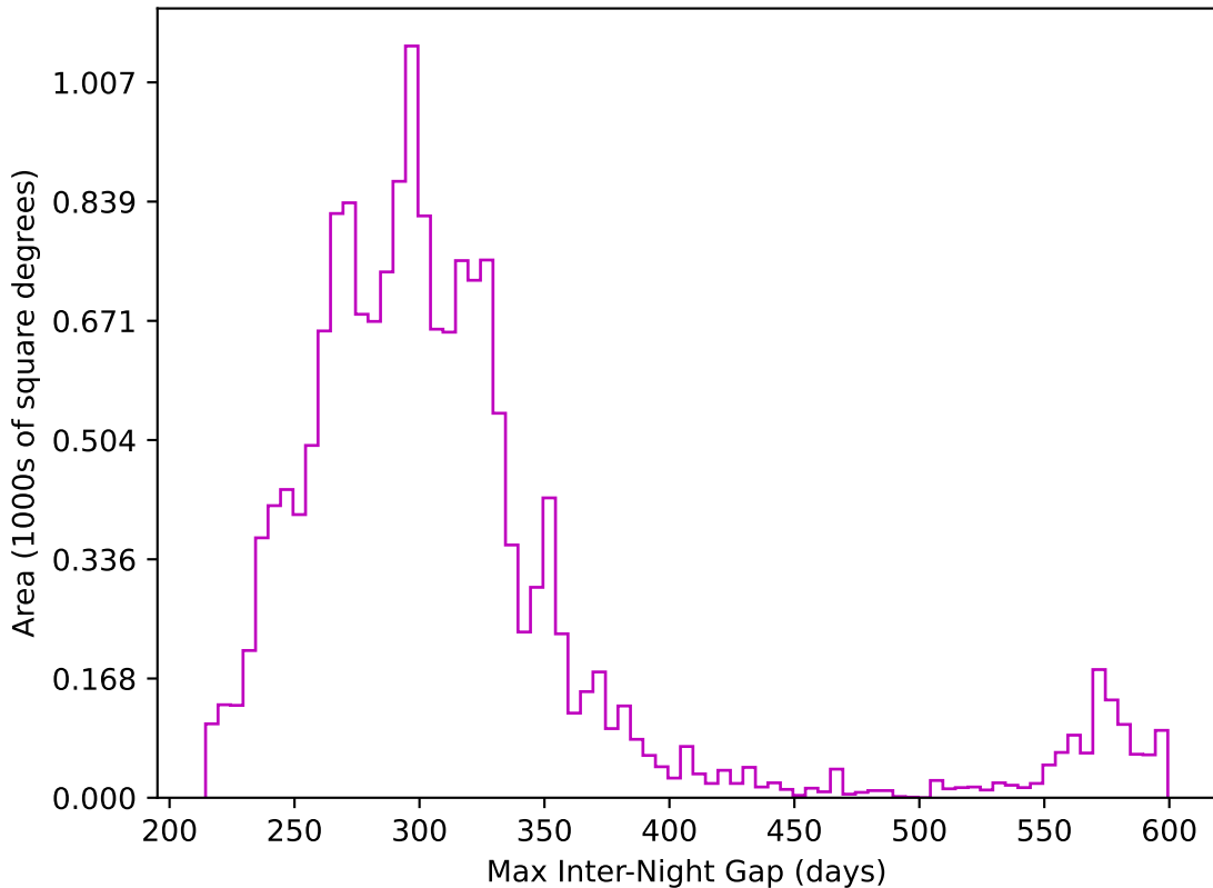
too_elab_heavy_r32_d3_gz_v3.4_10yrs WFD z band: Max Inter-Night Gap
