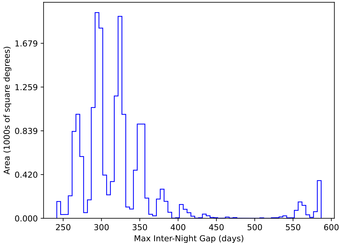
too_elab_heavy_r32_d3_gz_v3.4_10yrs WFD y band: Max Inter-Night Gap
