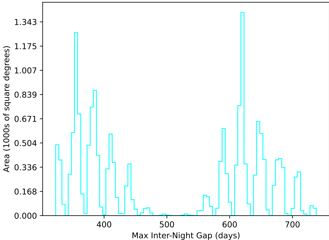
too_elab_heavy_r32_d3_gz_v3.4_10yrs WFD u band: Max Inter-Night Gap
