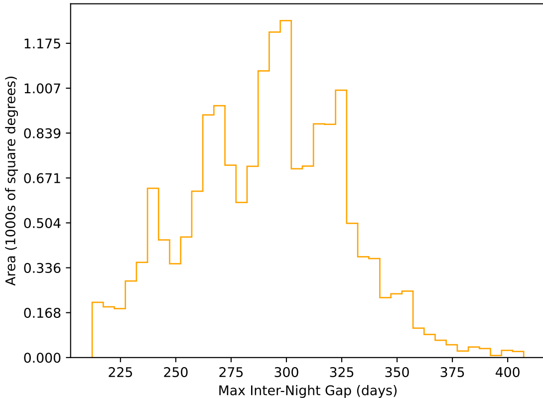
too_elab_heavy_r32_d3_gz_v3.4_10yrs WFD r band: Max Inter-Night Gap
