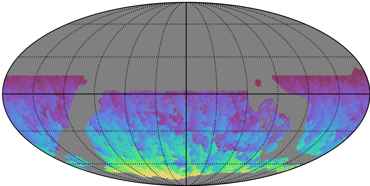
too_elab_heavy_r32_d3_gz_v3.4_10yrs WFD y band: Max HA
