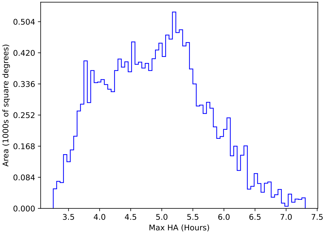
too_elab_heavy_r32_d3_gz_v3.4_10yrs WFD i band: Max HA
