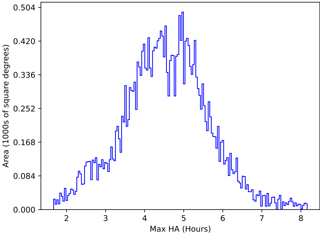
too_elab_heavy_r32_d3_gz_v3.4_10yrs All sky z band: Max HA
