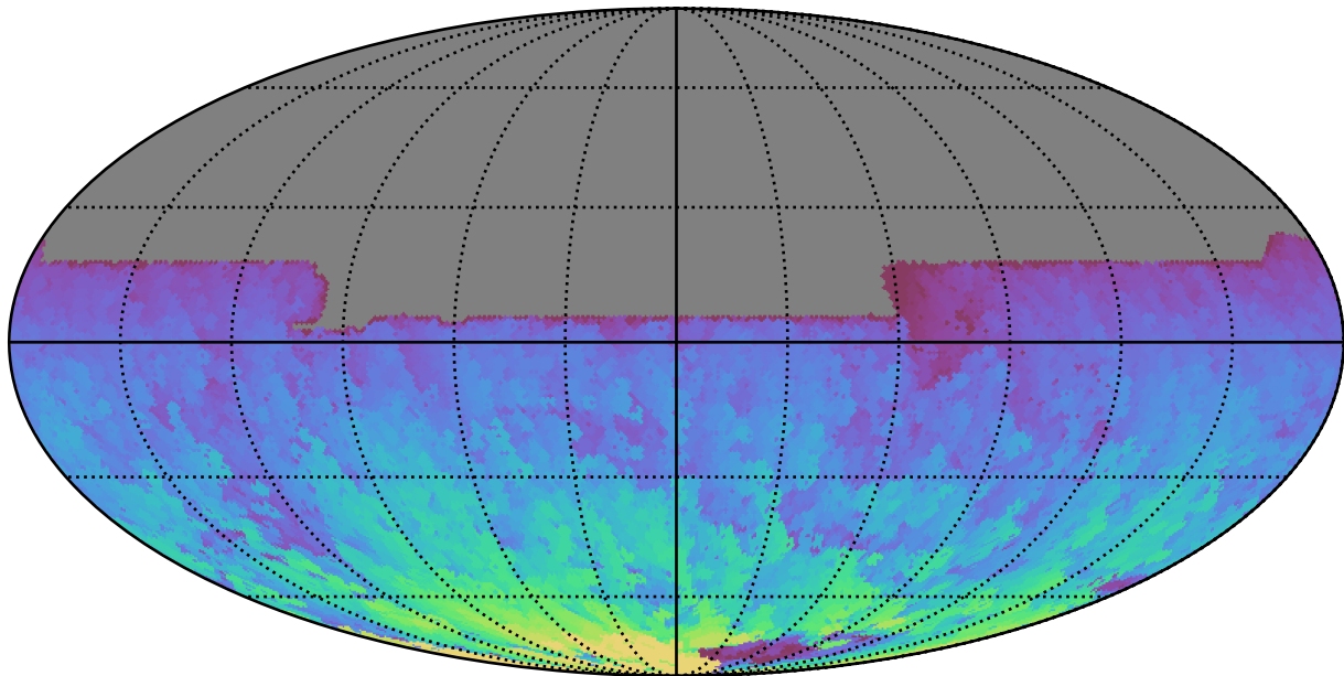
too_elab_heavy_r32_d3_gz_v3.4_10yrs All sky y band: Max HA
