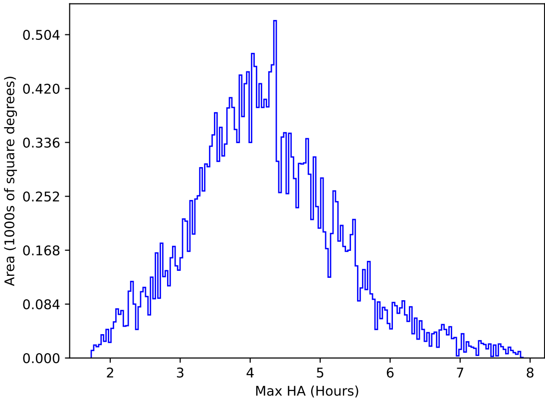
too_elab_heavy_r32_d3_gz_v3.4_10yrs All sky r band: Max HA
