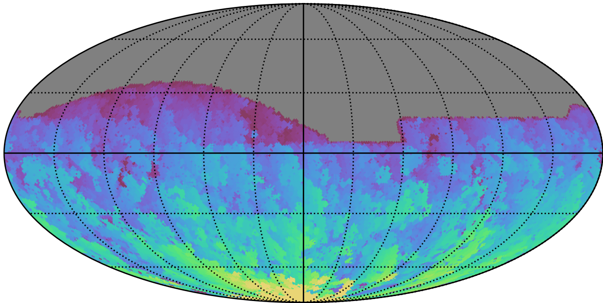
too_elab_heavy_r32_d3_gz_v3.4_10yrs All sky g band: Max HA
