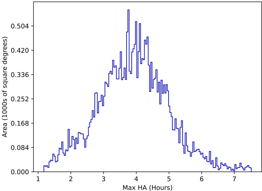
too_elab_heavy_r32_d3_gz_v3.4_10yrs All sky g band: Max HA
