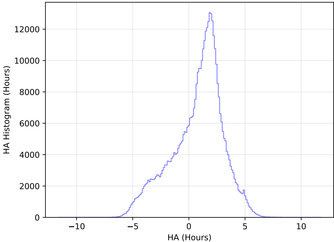
too_elab_heavy_r32_d3_gz_v3.4_10yrs WFD z band: HA Histogram
