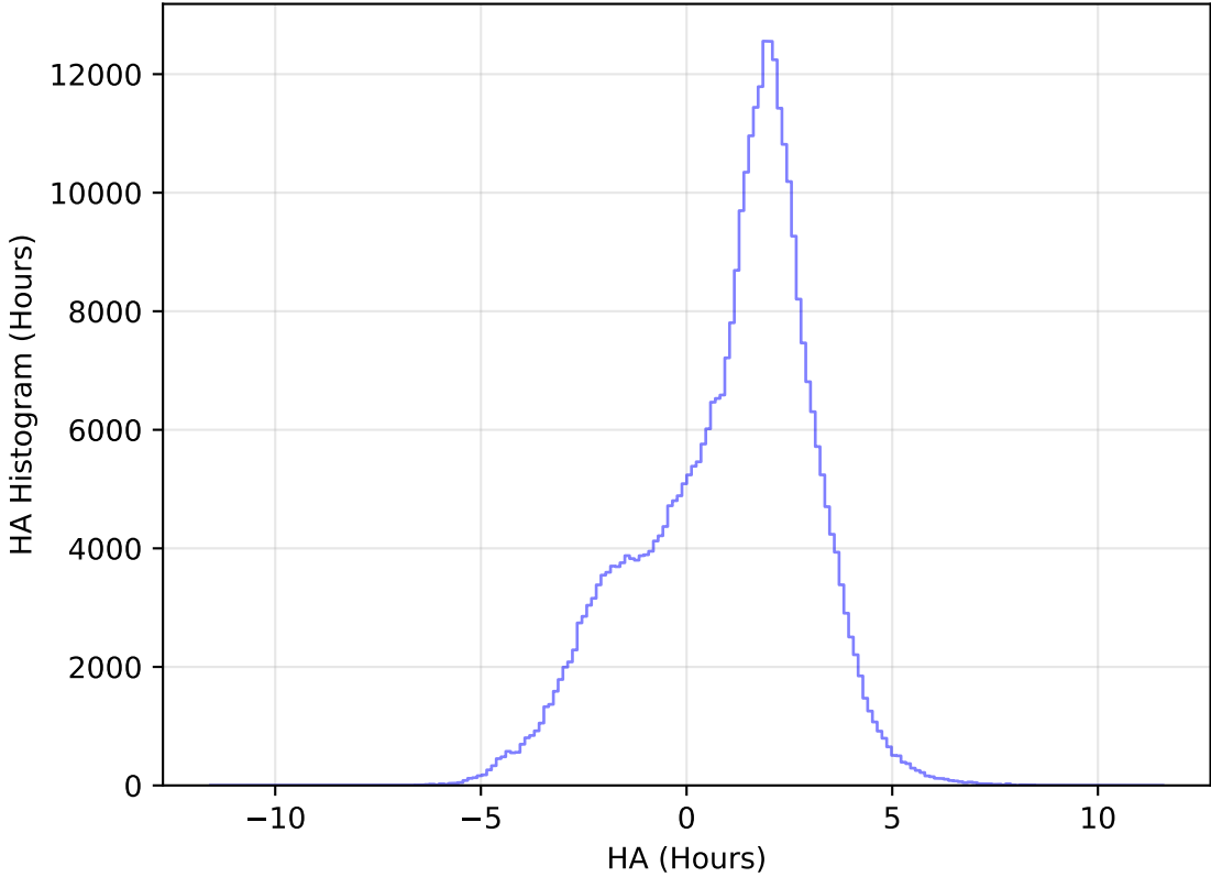
too_elab_heavy_r32_d3_gz_v3.4_10yrs WFD y band: HA Histogram
