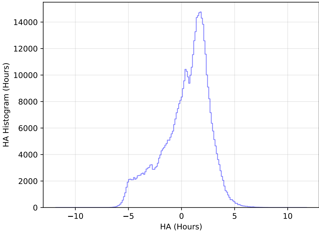
too_elab_heavy_r32_d3_gz_v3.4_10yrs WFD r band: HA Histogram
