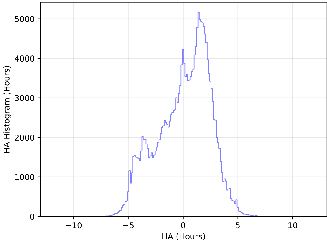
too_elab_heavy_r32_d3_gz_v3.4_10yrs WFD g band: HA Histogram
