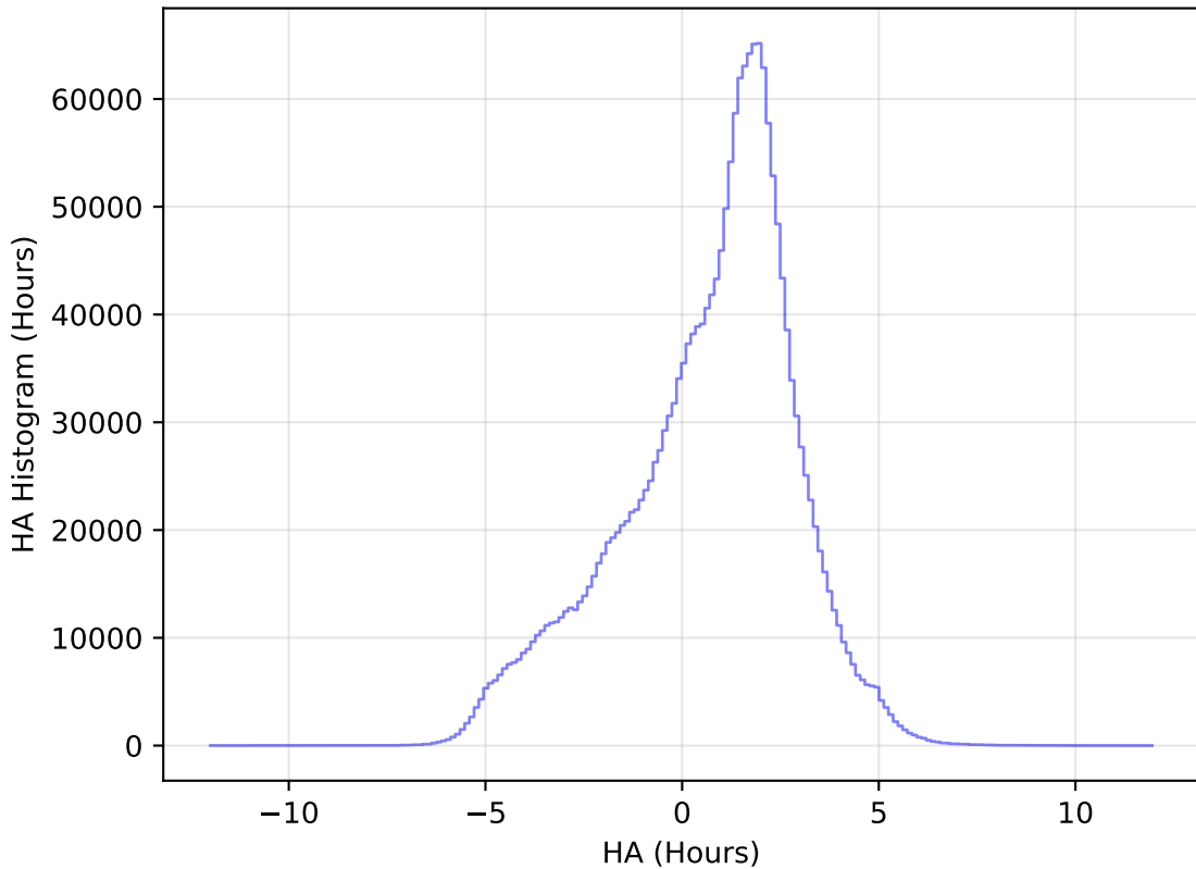
too_elab_heavy_r32_d3_gz_v3.4_10yrs WFD all bands: HA Histogram
