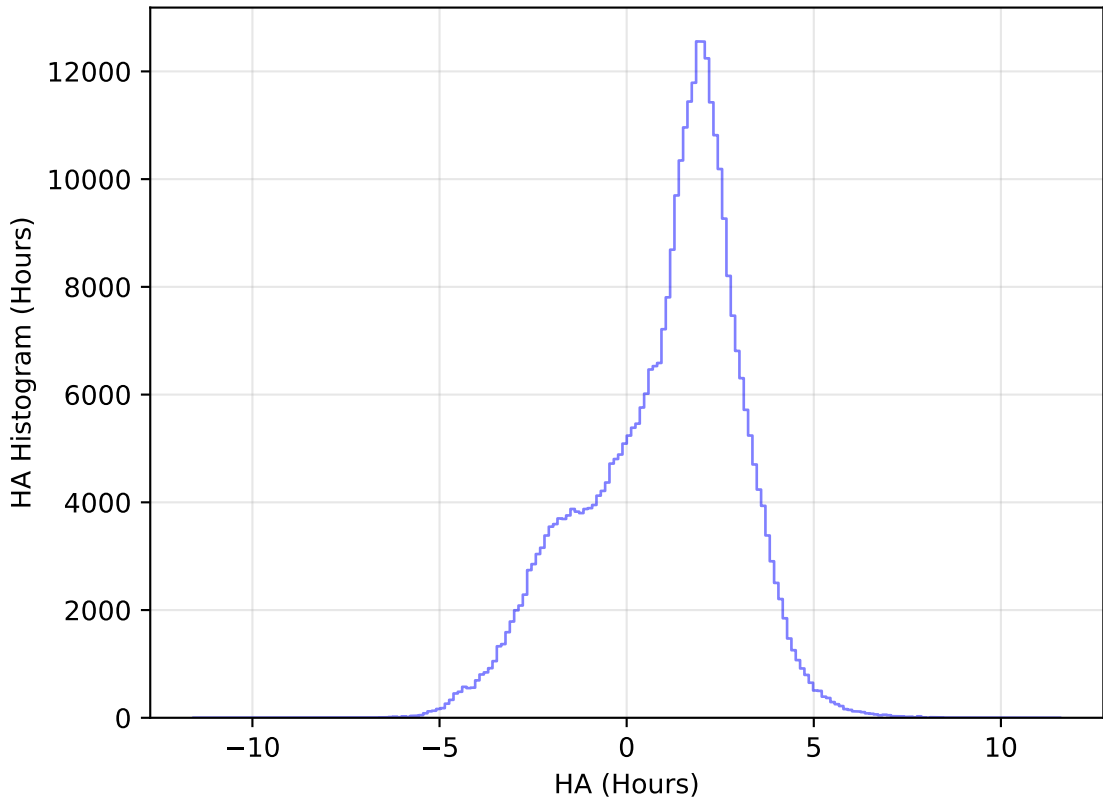
too_elab_heavy_r32_d3_gz_v3.4_10yrs All sky y band: HA Histogram
