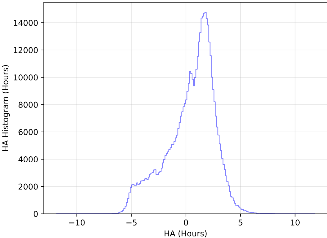
too_elab_heavy_r32_d3_gz_v3.4_10yrs All sky r band: HA Histogram
