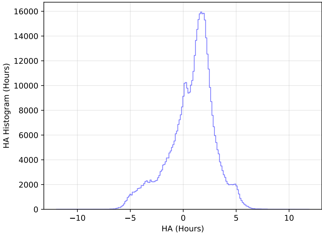
too_elab_heavy_r32_d3_gz_v3.4_10yrs All sky i band: HA Histogram
