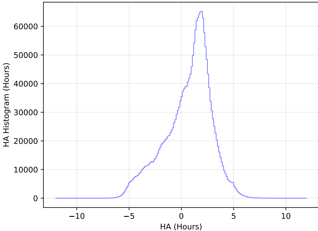
too_elab_heavy_r32_d3_gz_v3.4_10yrs All sky all bands: HA Histogram
