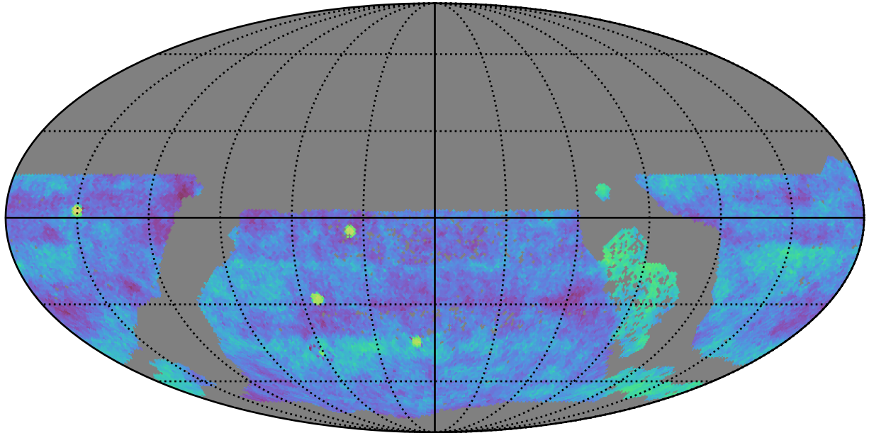
too_elab_heavy_r32_d3_gz_v3.4_10yrs gri WFD: Fraction of visits in pairs (20-90 min)
