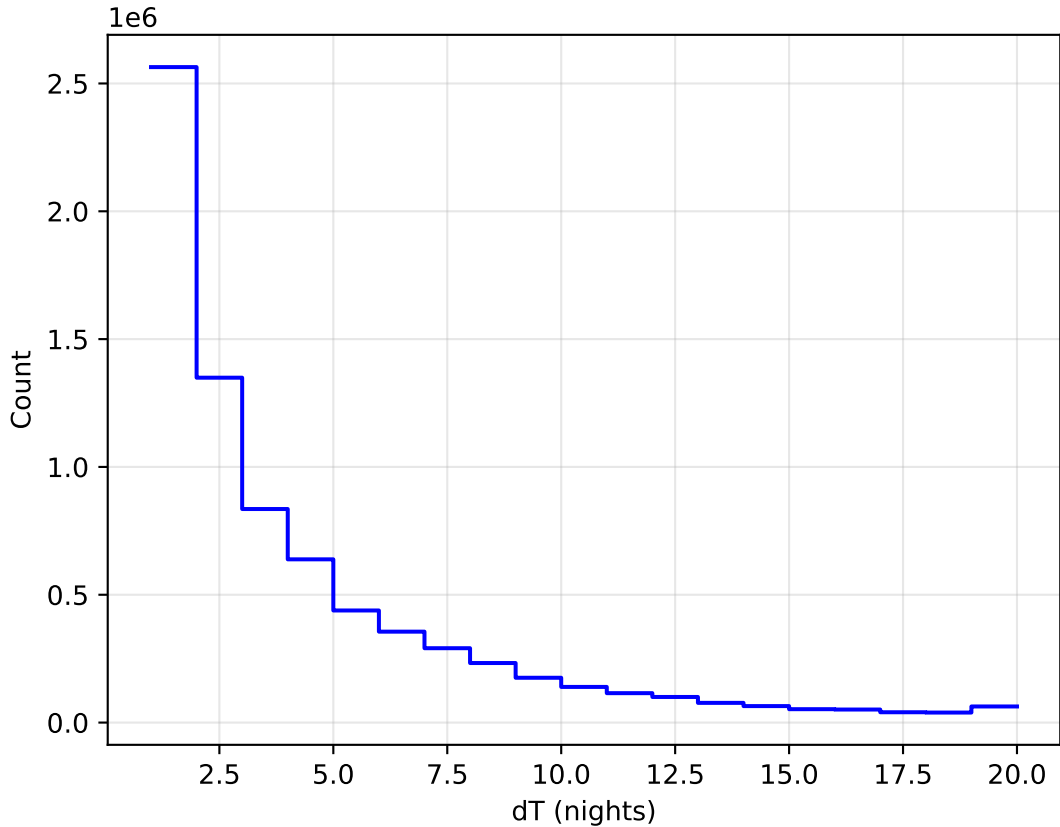
too_elab_heavy_r32_d3_gz_v3.4_10yrs WFD all bands: DeltaNight Histogram
