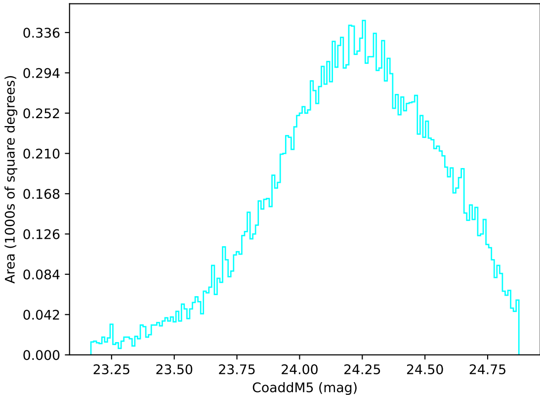
too_elab_heavy_r32_d3_gz_v3.4_10yrs Yr 1 u band: CoaddM5
