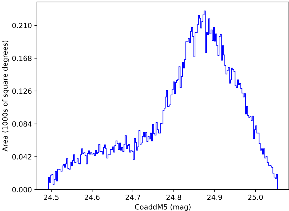
too_elab_heavy_r32_d3_gz_v3.4_10yrs WFD y band: CoaddM5
