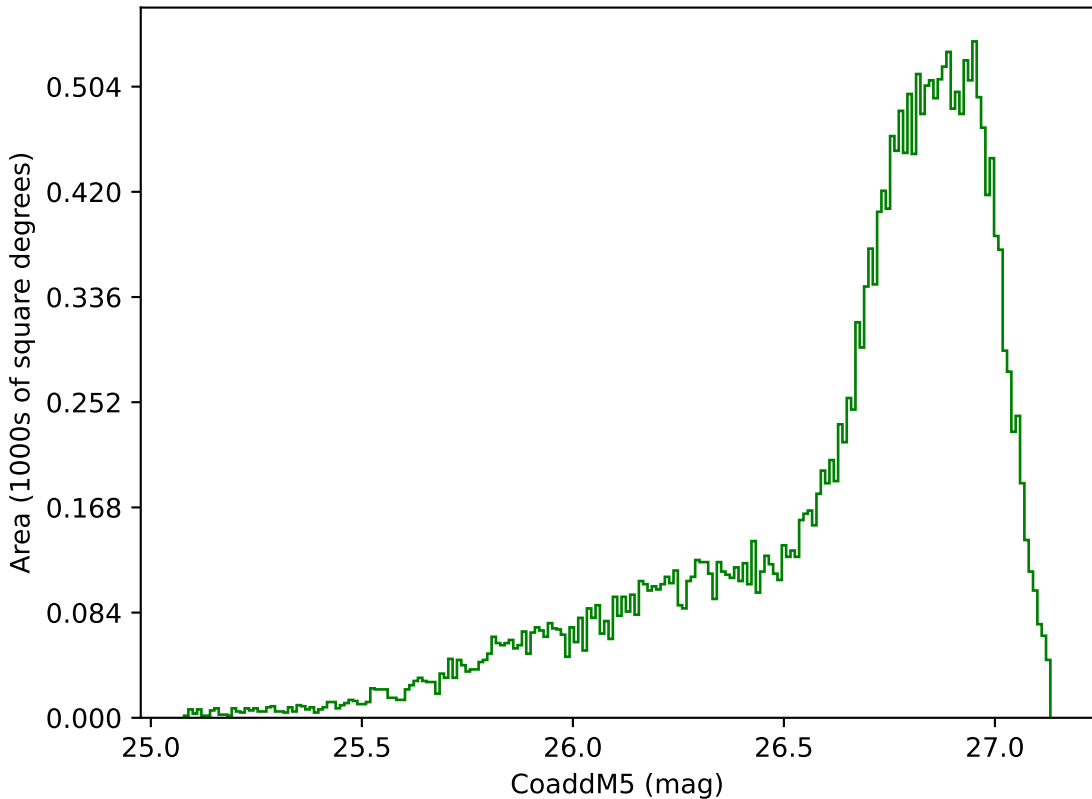
too_elab_heavy_r32_d3_gz_v3.4_10yrs All sky g band: CoaddM5
