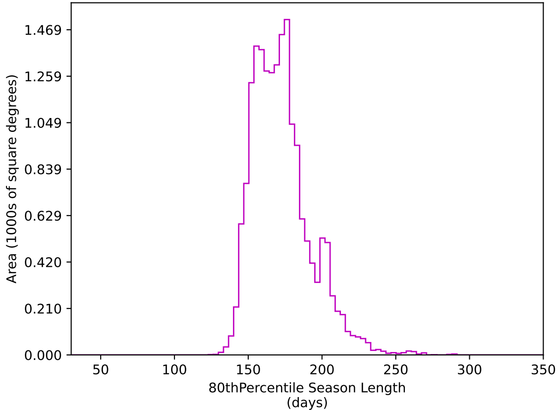
too_elab_heavy_r32_d3_gz_v3.4_10yrs WFD z band: 80thPercentile Season Length
