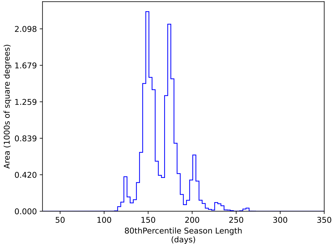
too_elab_heavy_r32_d3_gz_v3.4_10yrs WFD y band: 80thPercentile Season Length
