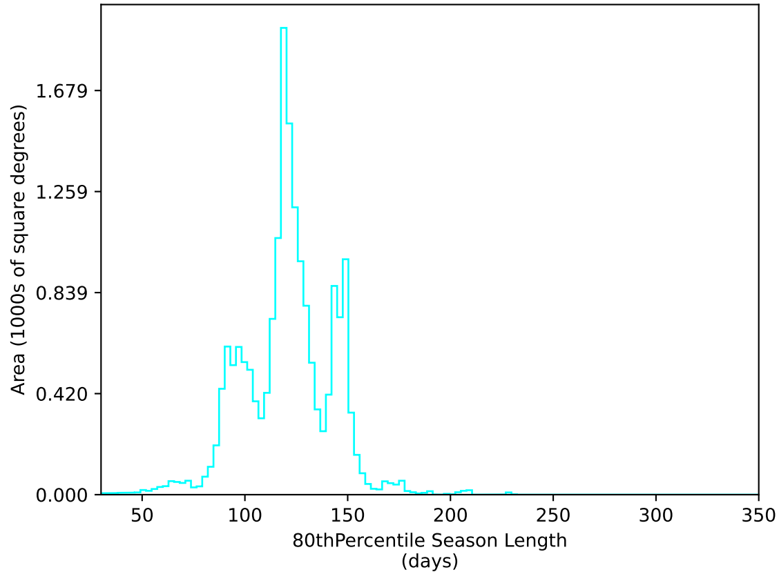
too_elab_heavy_r32_d3_gz_v3.4_10yrs WFD u band: 80thPercentile Season Length
