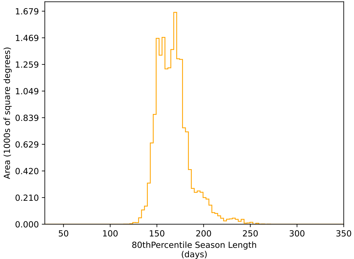
too_elab_heavy_r32_d3_gz_v3.4_10yrs WFD r band: 80thPercentile Season Length
