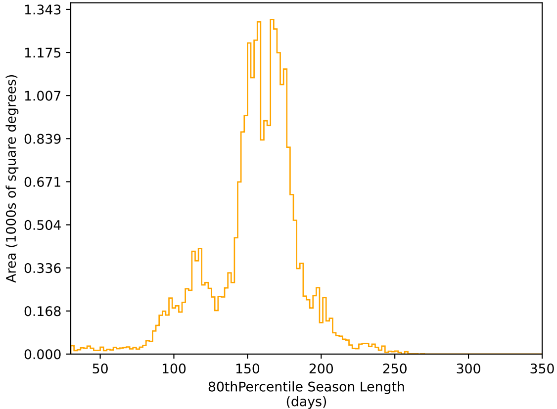
too_elab_heavy_r32_d3_gz_v3.4_10yrs All sky r band: 80thPercentile Season Length
