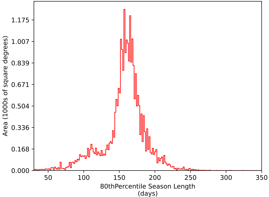
too_elab_heavy_r32_d3_gz_v3.4_10yrs All sky i band: 80thPercentile Season Length
