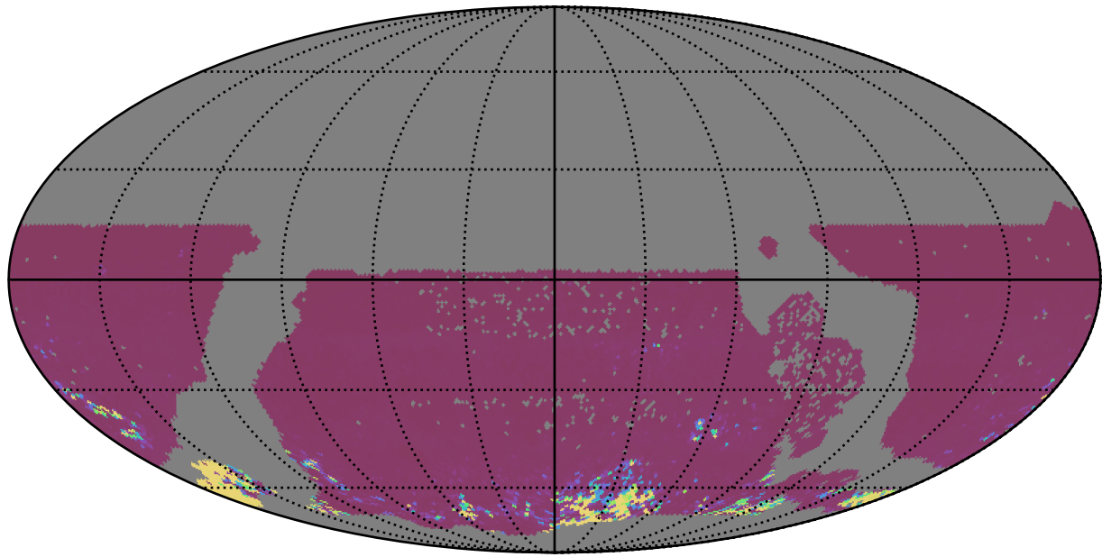
too_elab_heavy_r32_d3_gz_v3.4_10yrs WFD ri bands: 75th Percentile Intranight Timespan
