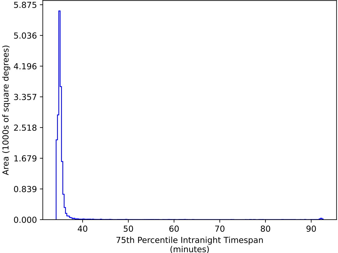
too_elab_heavy_r32_d3_gz_v3.4_10yrs WFD ri bands: 75th Percentile Intranight Timespan
