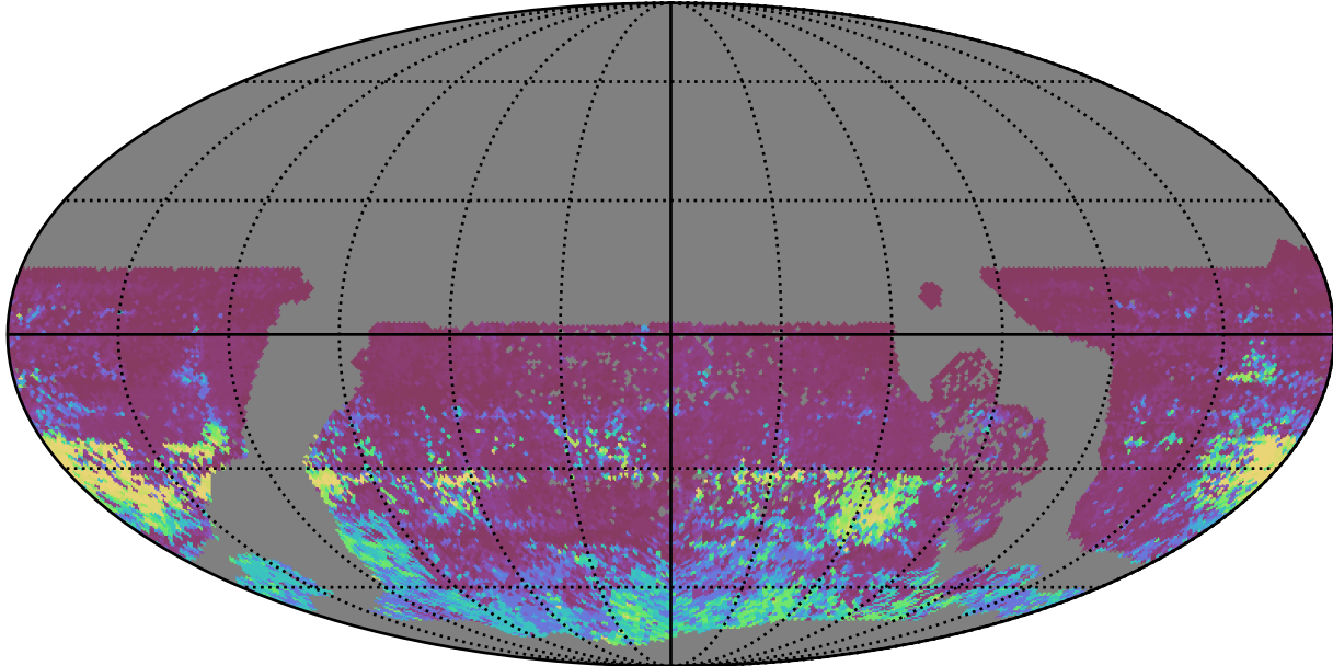
too_elab_heavy_r32_d3_gz_v3.4_10yrs WFD r band: 75th Percentile Intranight Timespan
