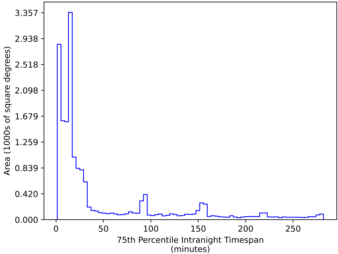
too_elab_heavy_r32_d3_gz_v3.4_10yrs WFD r band: 75th Percentile Intranight Timespan
