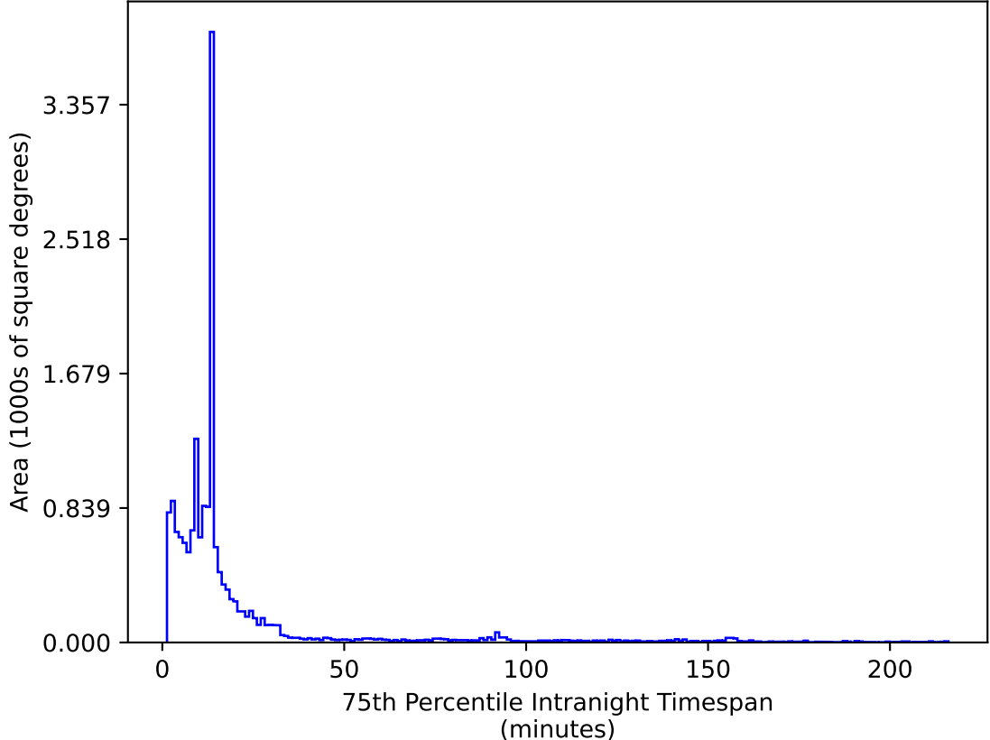
too_elab_heavy_r32_d3_gz_v3.4_10yrs WFD i band: 75th Percentile Intranight Timespan
