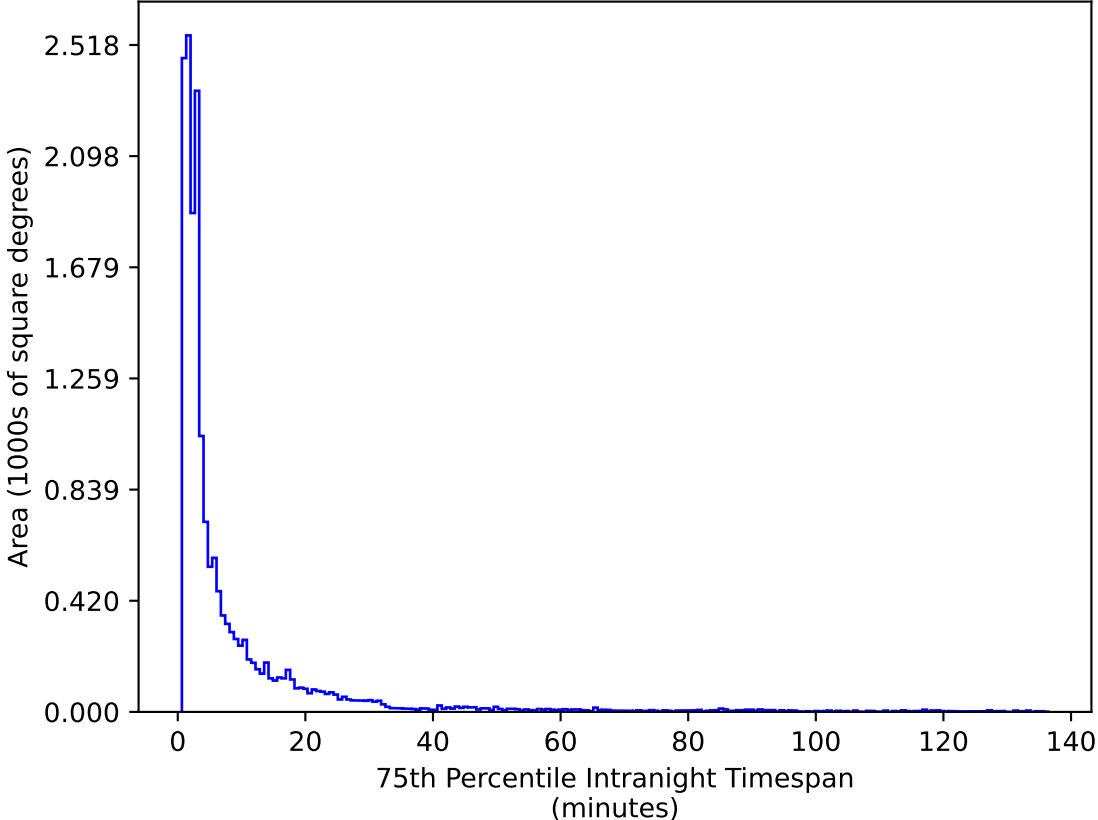
too_elab_heavy_r32_d3_gz_v3.4_10yrs WFD g band: 75th Percentile Intranight Timespan
