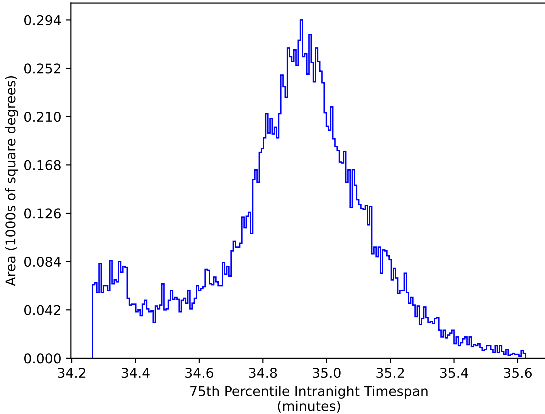
too_elab_heavy_r32_d3_gz_v3.4_10yrs WFD all bands: 75th Percentile Intranight Timespan
