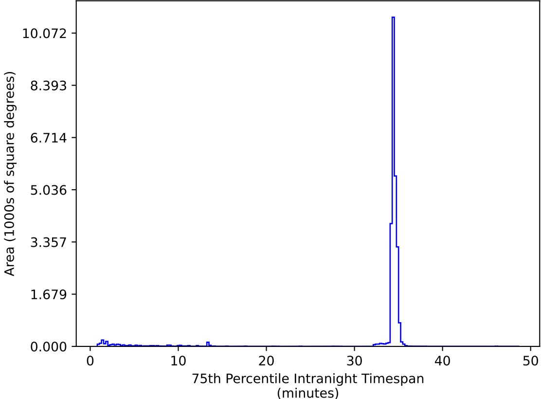
too_elab_heavy_r32_d3_gz_v3.4_10yrs All sky zy bands: 75th Percentile Intranight Timespan
