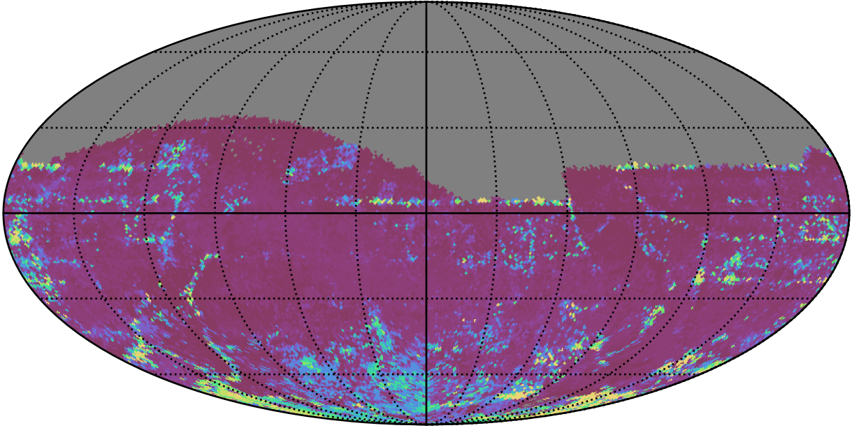
too_elab_heavy_r32_d3_gz_v3.4_10yrs All sky z band: 75th Percentile Intranight Timespan
