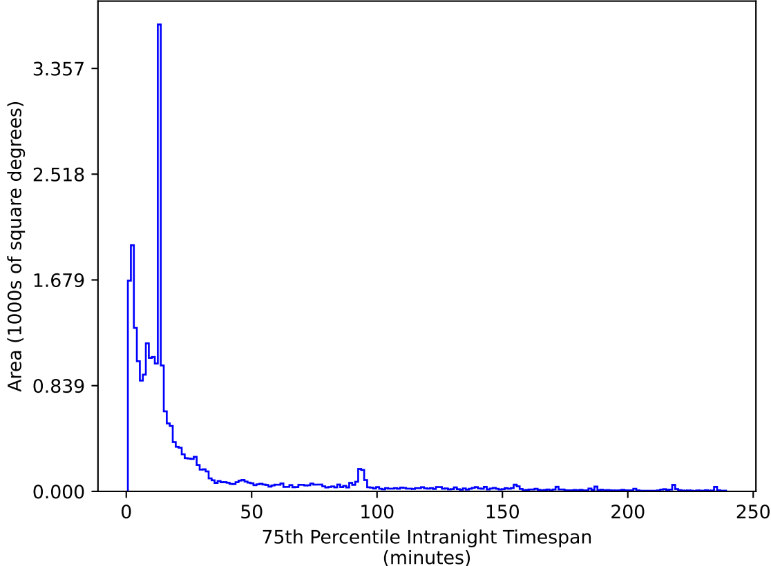
too_elab_heavy_r32_d3_gz_v3.4_10yrs All sky z band: 75th Percentile Intranight Timespan
