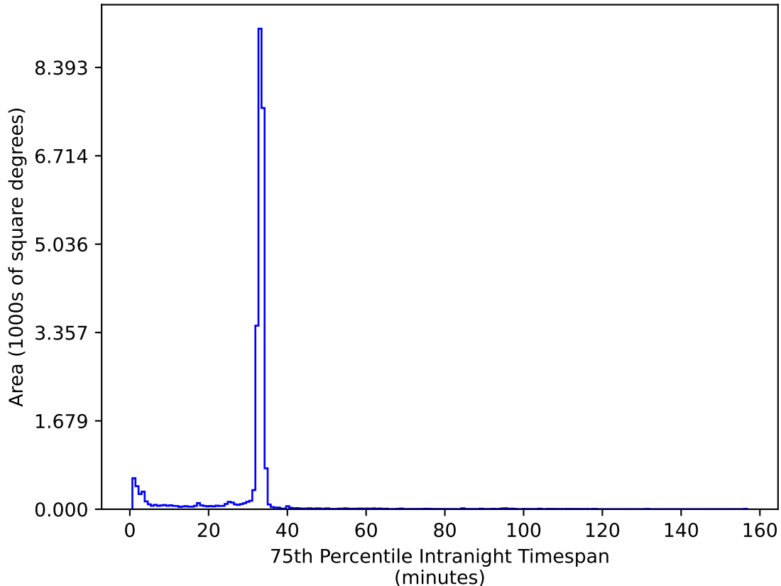
too_elab_heavy_r32_d3_gz_v3.4_10yrs All sky ug bands: 75th Percentile Intranight Timespan
