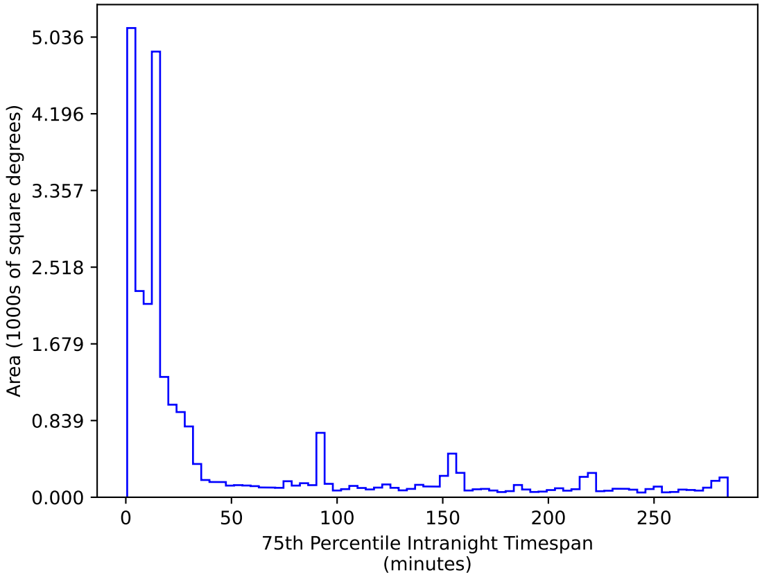
too_elab_heavy_r32_d3_gz_v3.4_10yrs All sky r band: 75th Percentile Intranight Timespan
