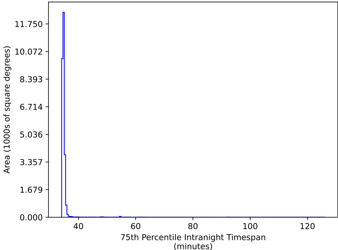
too_elab_heavy_r32_d3_gz_v3.4_10yrs All sky iz bands: 75th Percentile Intranight Timespan
