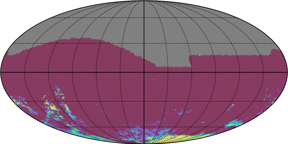
too_elab_heavy_r32_d3_gz_v3.4_10yrs All sky gr bands: 75th Percentile Intranight Timespan
