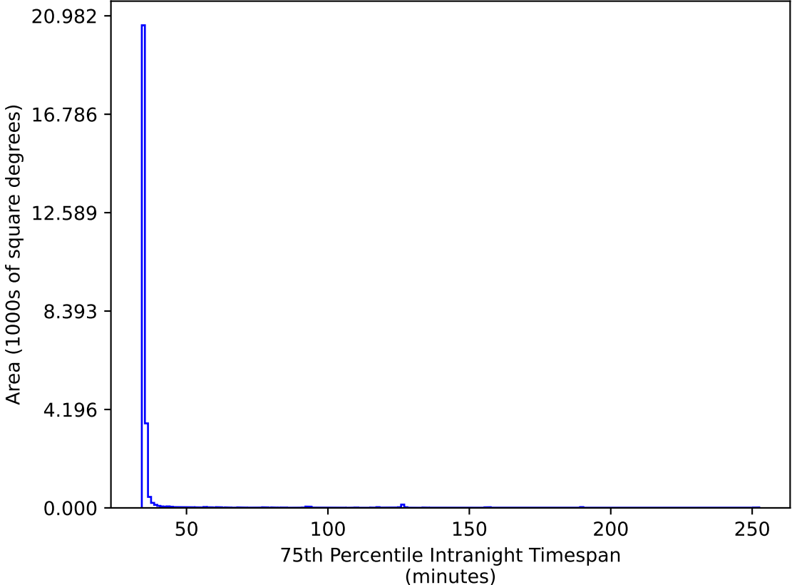
too_elab_heavy_r32_d3_gz_v3.4_10yrs All sky gr bands: 75th Percentile Intranight Timespan
