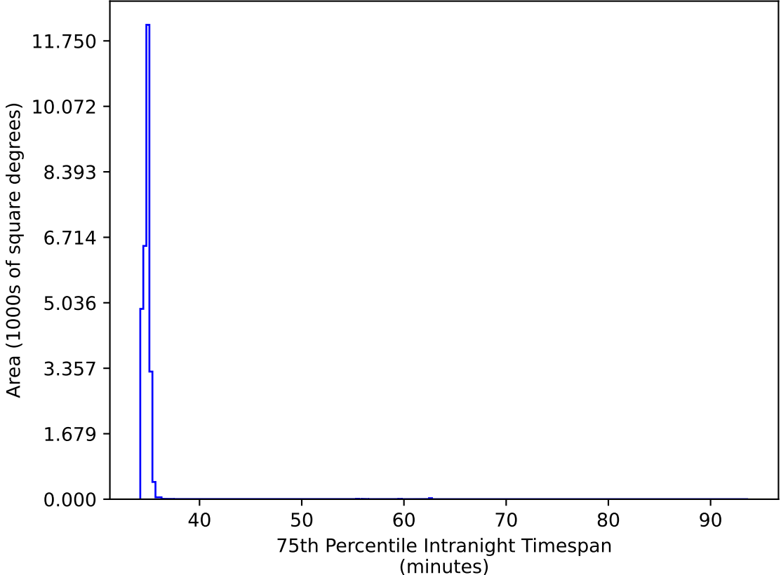
too_elab_heavy_r32_d3_gz_v3.4_10yrs All sky all bands: 75th Percentile Intranight Timespan
