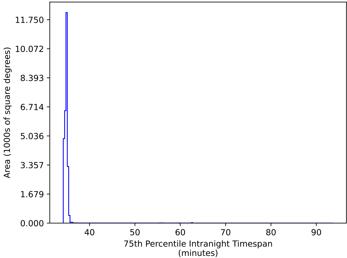
too_elab_heavy_r32_d3_gz_v3.4_10yrs All sky: 75th Percentile Intranight Timespan
