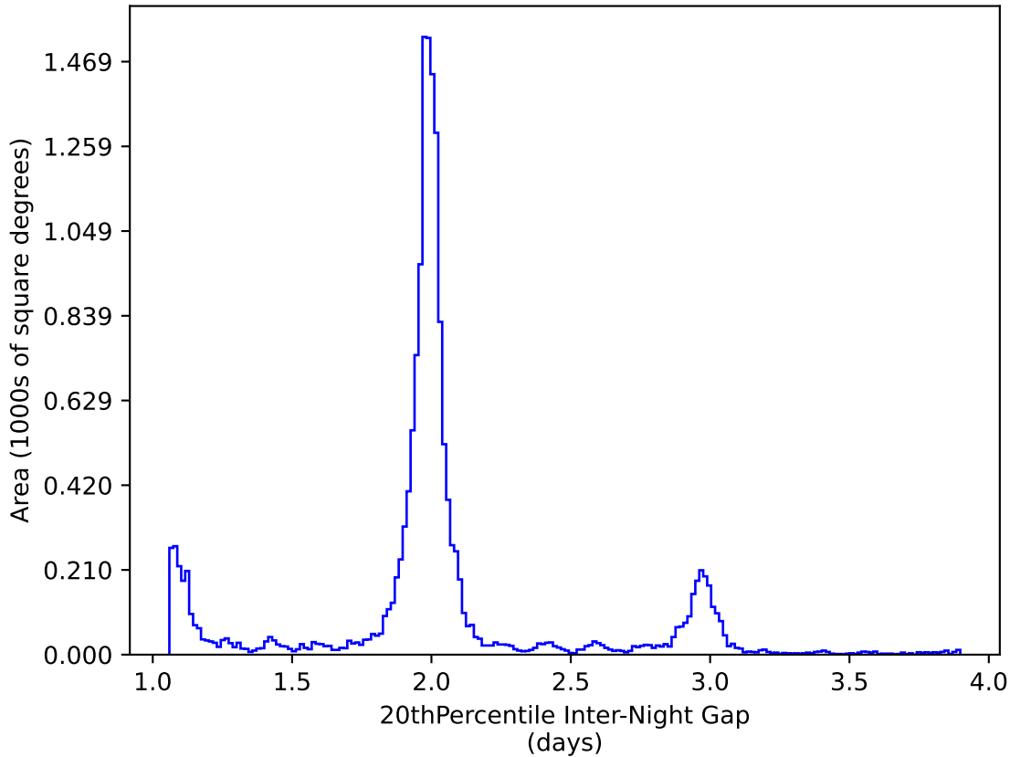
too_elab_heavy_r32_d3_gz_v3.4_10yrs WFD y band: 20thPercentile Inter-Night Gap
