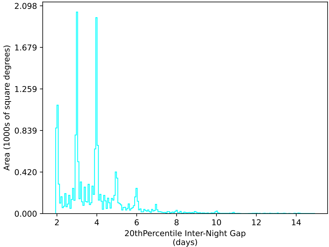
too_elab_heavy_r32_d3_gz_v3.4_10yrs WFD u band: 20thPercentile Inter-Night Gap
